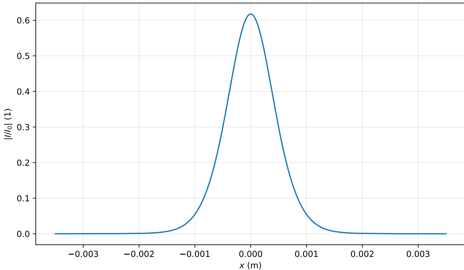
Intensity profile I(x, y = 0, z = 3.264m)/I_0 , P_{in}=0.6P_{cr} , artificial time
